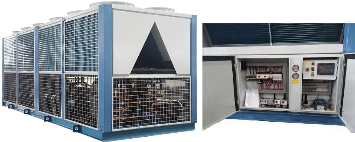
Air cooled screw compressor
